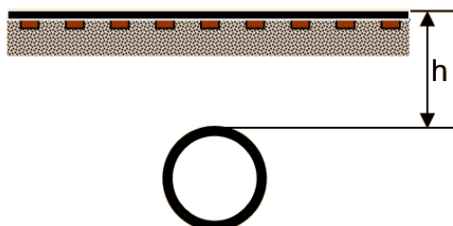
Figure 2.7 : Couverture minimale
