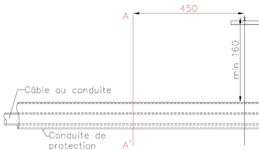
Figure 2.8 : Distance minimale
