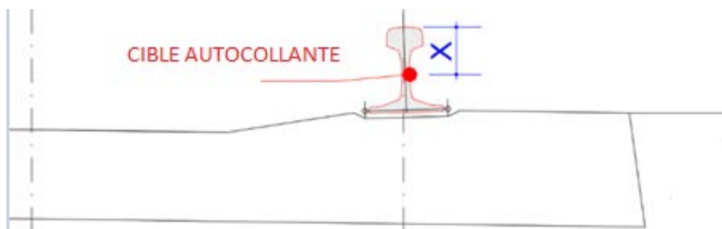
Figure 2.11 - Placement de cible
